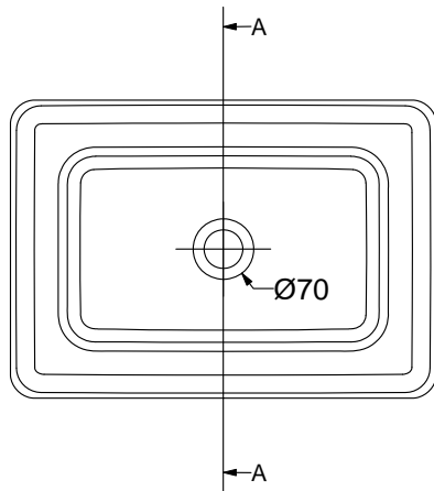
C BOTTOM_VIEW
